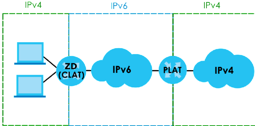
Figure 64 464XLAT
