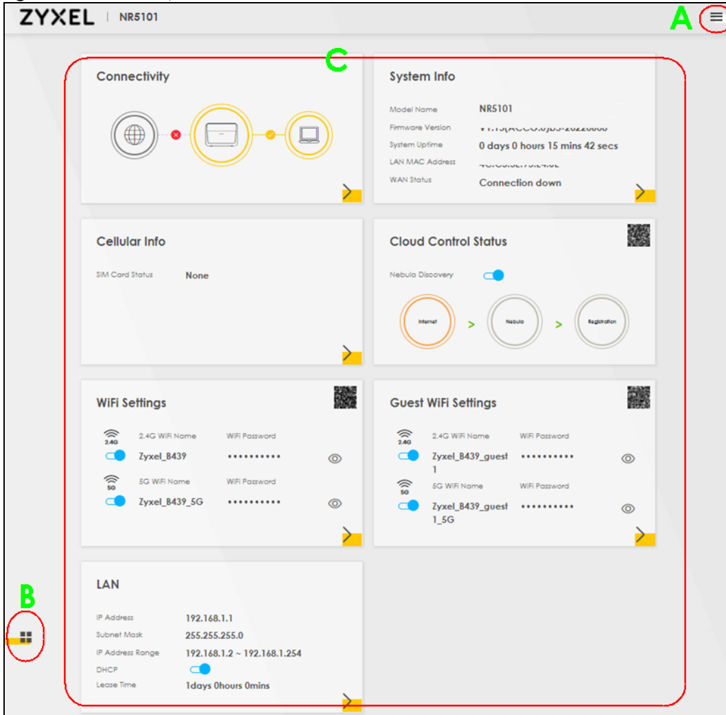
Figure 37 Screen Layout
