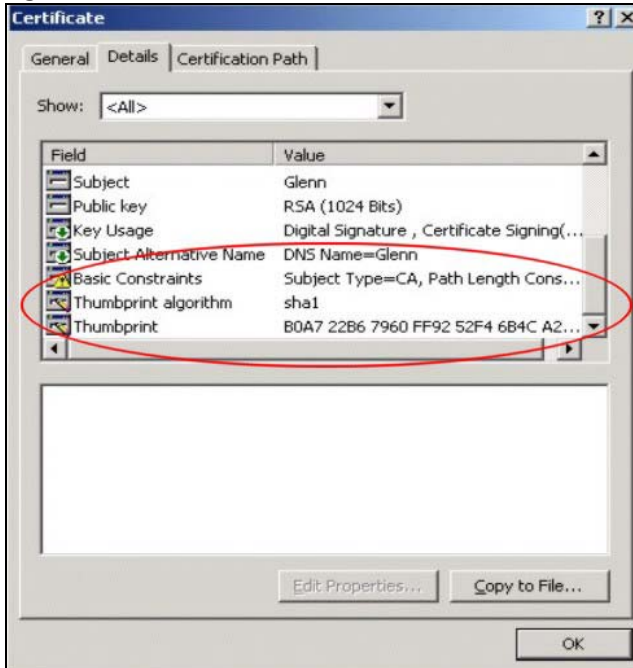
Figure 170 Certificate Details
