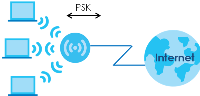
Figure 221 WPA(2)-PSK Authentication
