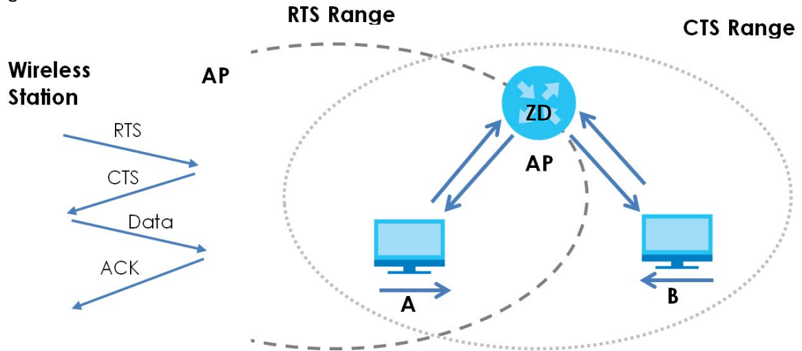
Figure 219 RTS/CTS
