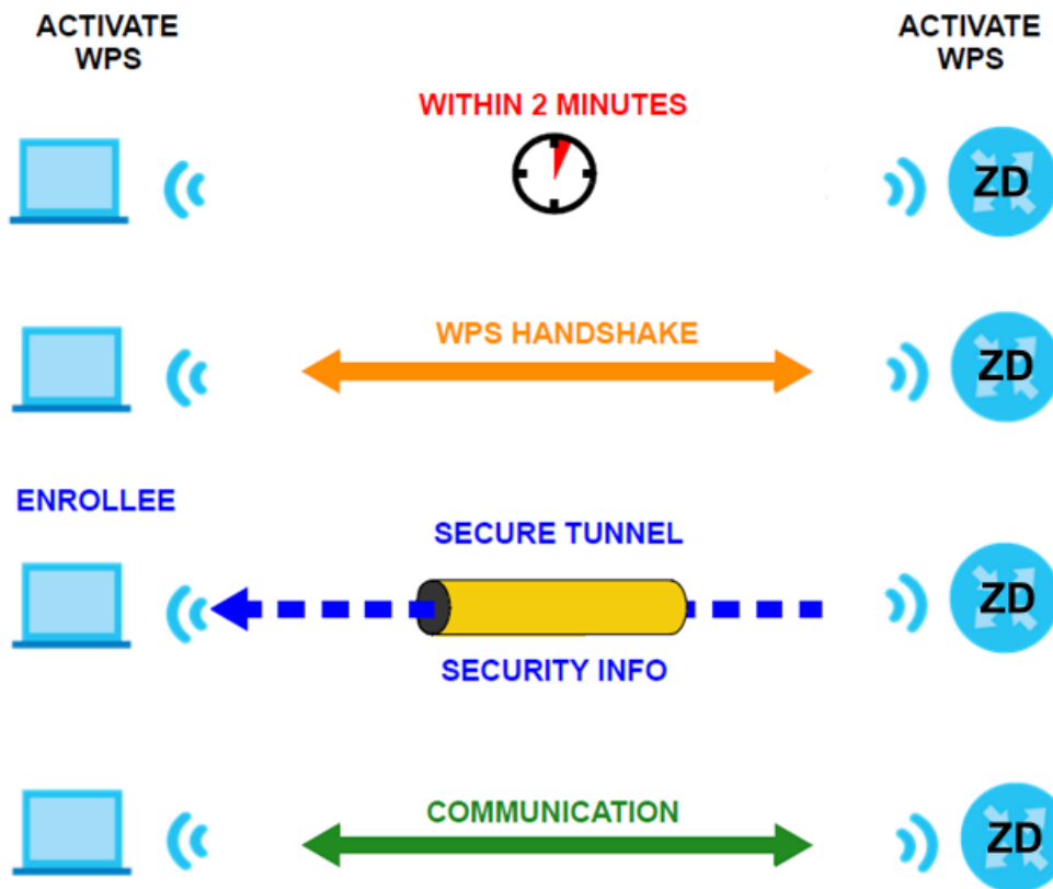
Figure 100 How WPS Works
