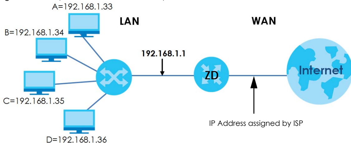
Figure 139 Multiple Servers Behind NAT Example
