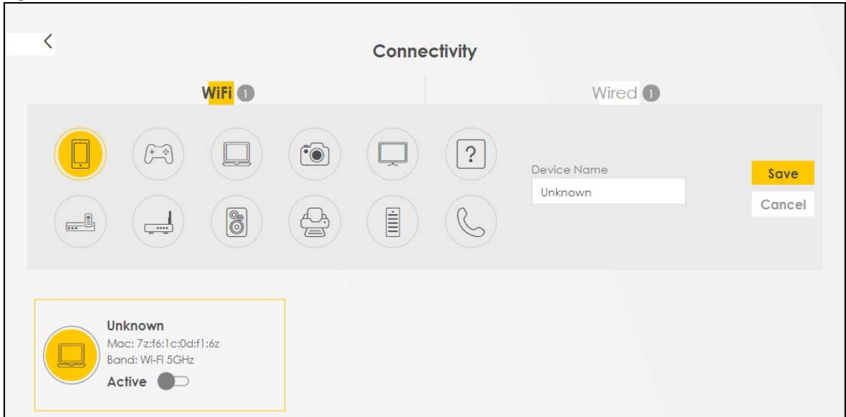
Figure 49 Connectivity: Edit
