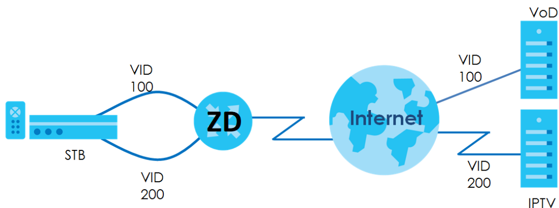
Figure 143 VLAN Group Example
