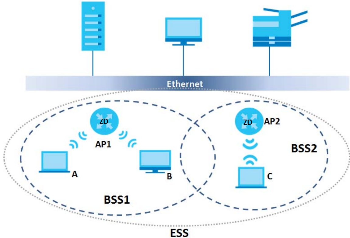
Figure 218 Infrastructure WLAN
